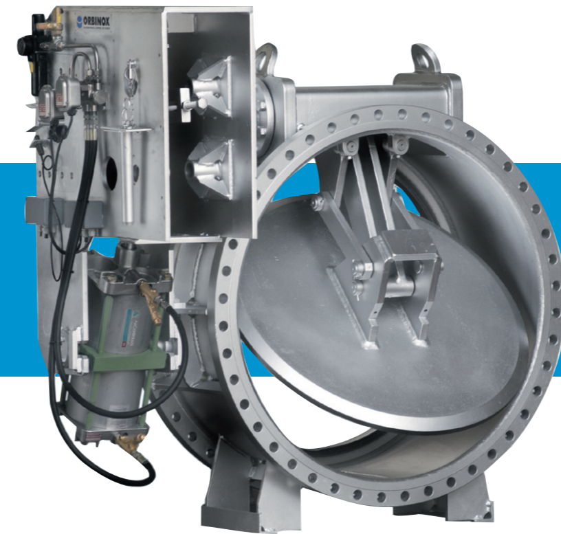
MP Válvula de triple palanca. Three-lever valve. Dreihebelklappe.
