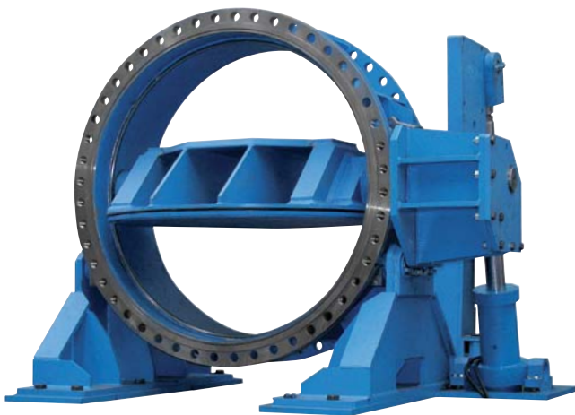
MB Double Eccentric Butterfly Valve
